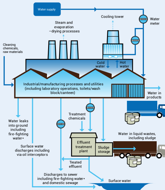
Water inputs and outputs for an example industrial site
