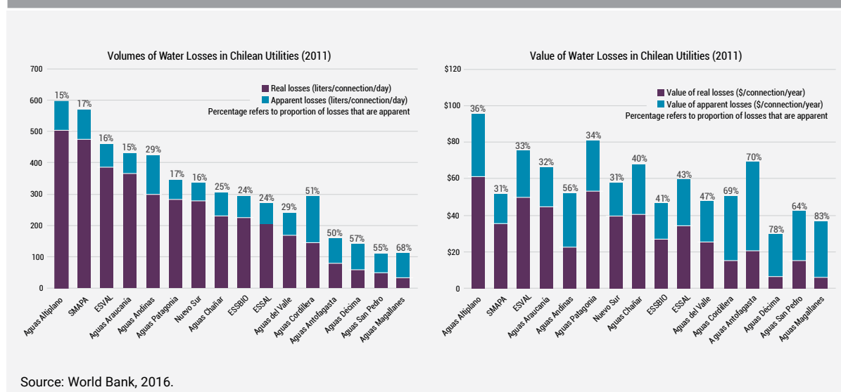
FIGURE 5: VOLUME AND VALUES OF WATER LOSSES IN CHILEAN WATER UTILITIES IN 2011
