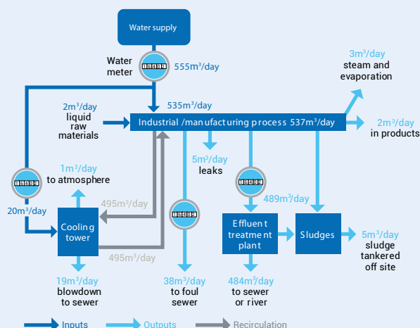
Water use in food manufacture
