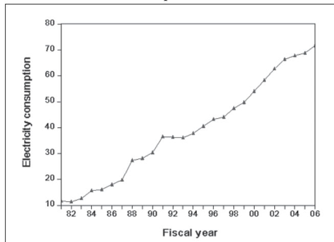
Figure 2. Historical Trend of Per Capita Electricity Consumption of Nepal (in kWh)
