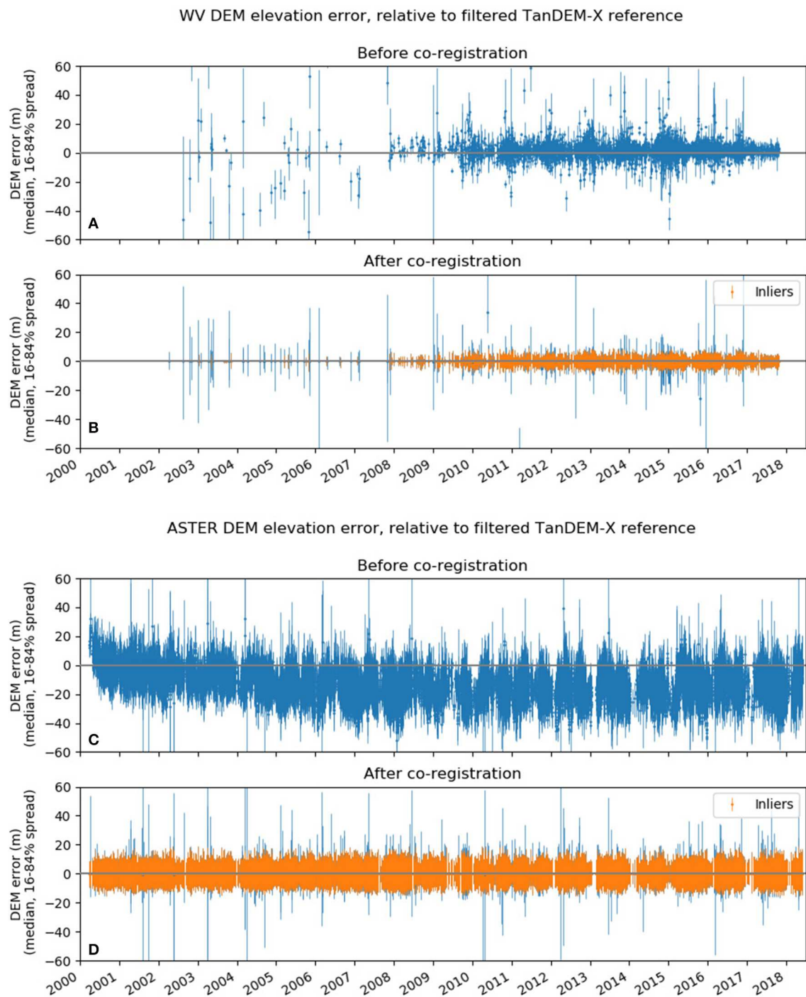
FIGURE 2 | Temporal coverage and error metrics for WorldView/GeoEye (A,B) and ASTER (C,D) DEMs before and after co-registration. Each point shows the median elevation offset between an individual DEM and the TanDEM-X Global DEM reference over surfaces assumed to be static. Error bars show the 16–84% spread of these elevation offset values for each DEM. The final set of DEMs used for subsequent analysis and trend-fitting are shown with orange points/bars (“inliers”). Note the apparent drift in median offsets throughout the ASTER mission (C), and zero bias after co-registration.
