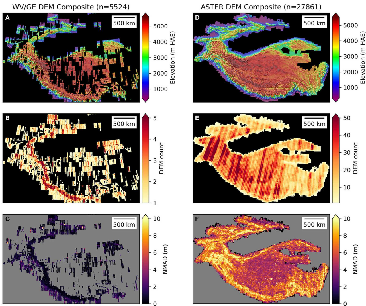
FIGURE 1 | Composite products for WorldView/GeoEye (A–C) and ASTER (D–F) DEMs after co-registration and quality control. Rows show per-pixel weighted mean, count, and normalized median absolute deviation (NMAD). Note difference in color ramp for count maps in B and E .
