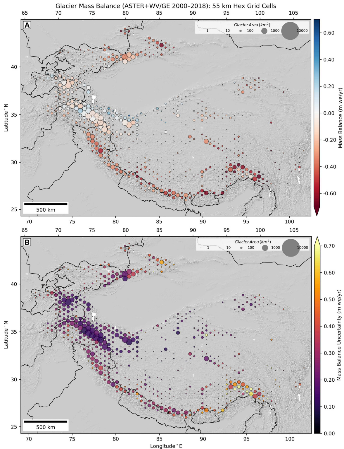
FIGURE 4 | (A) Specific glacier mass balance ( \text{m w.e. yr}^{-1} ) and (B) uncertainty for the period from 2000 to 2018, aggregated over 55 km hex grid cells. The size of the circle for each cell is scaled by total glacierized area within that cell. Approximate international borders from Natural Earth 1:10M products are plotted for reference. See Figure S4 for units of \text{Gt yr}^{-1} .
