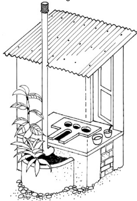
Figure 3: Kerala double vault dehydration toilet [Illustrator: Hans Mårtensson; Source: Winblad and Simpson-Hébert, 2004]
