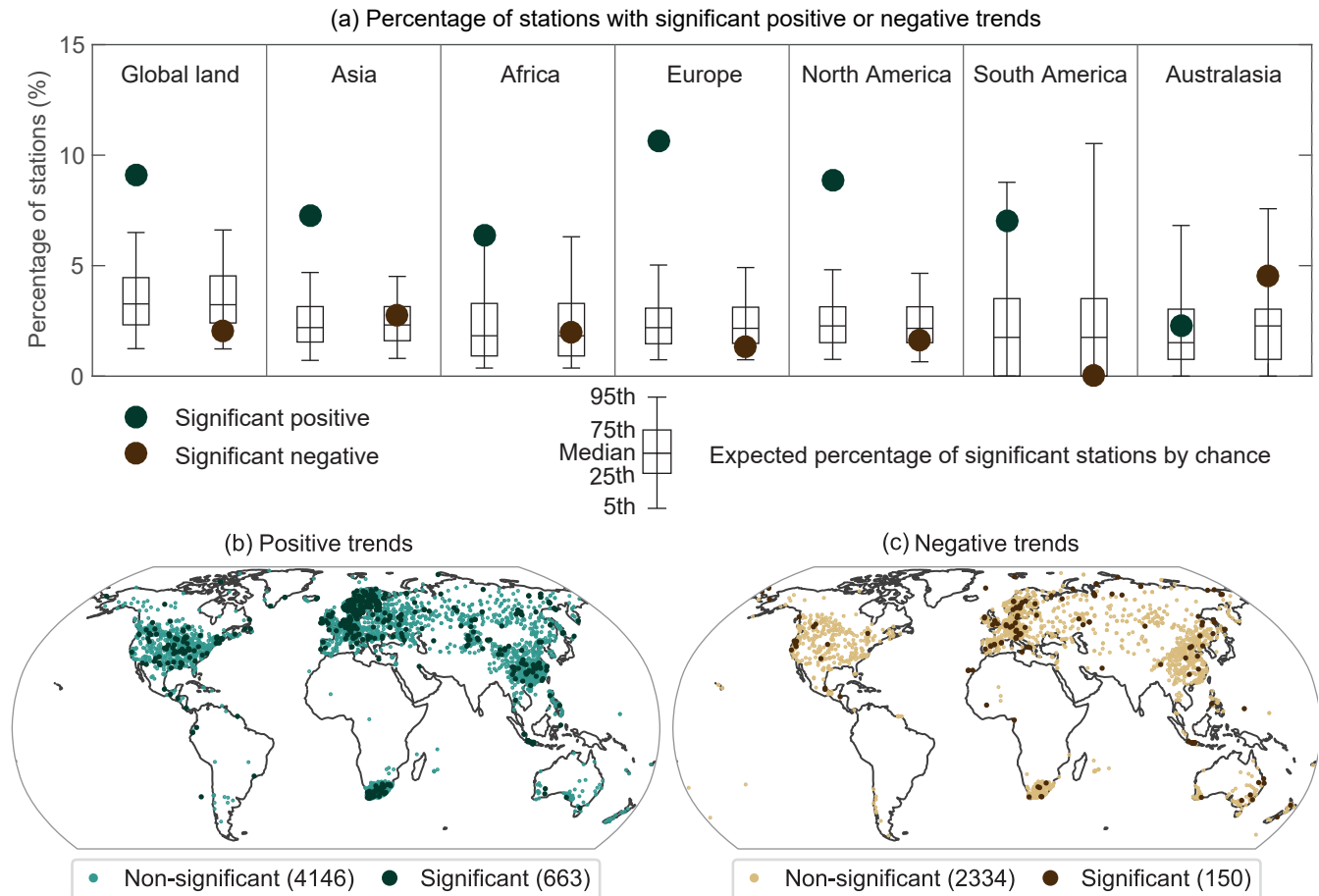
Figure 11.13 | Signs and significance of the observed trends in annual maximum daily precipitation (Rx1day) during 1950–2018 at 8345 stations with sufficient data. (a) Percentage of stations with statistically significant trends in Rx1day; green dots show positive trends and brown dots negative trends. Box and 'whisker' plots indicate the expected percentage of stations with significant trends due to chance estimated from 1000 bootstrap realizations under a no-trend null hypothesis. The boxes mark the median, 25th percentile, and 75th percentile. The upper and lower whiskers show the 97.5th and the 2.5th percentiles, respectively. Maps of stations with positive (b) and negative (c) trends. The light colour indicates stations with non-significant trends, and the dark colour stations with significant trends. Significance is determined by a two-tailed test conducted at the 5% level. Adapted from Sun et al. (2021). Figure copyright © American Meteorological Society (used with permission). Further details on data sources and processing are available in the chapter data table (Table 11.SM.9).
