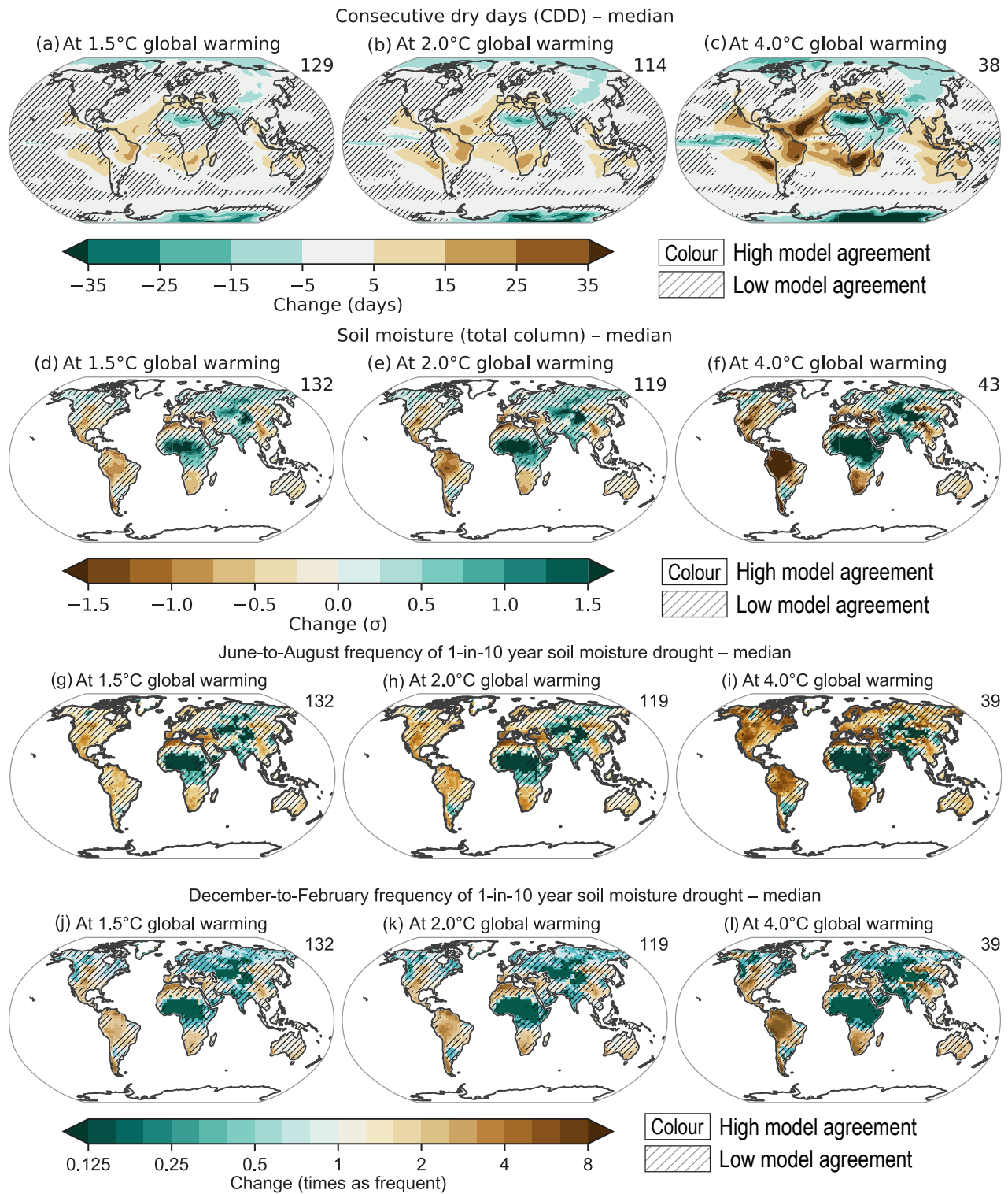
Figure 11.19 | Projected changes in (a–c) the number of consecutive dry days (CDD), (d–f) annual mean soil moisture over the total column, and (g–l) the frequency and intensity of 1-in-10-year soil moisture drought for the June-to-August and December-to-February seasons at 1.5°C, 2°C, and 4°C of global warming compared to the 1850–1900 baseline. The unit for soil moisture change is the standard deviation of interannual variability in soil moisture during 1850–1900. Standard deviation is a widely used metric in characterizing drought severity. A projected reduction in mean soil moisture by one standard deviation corresponds to soil moisture conditions typical of about 1-in-6-year droughts during 1850–1900 becoming the norm in the future. Results are based on simulations from the Coupled Model Intercomparison Project Phase 6 (CMIP6) multi-model ensemble under the Shared Socio-economic Pathway (SSP), SSP1-1.9, SSP1-2.6, SSP2-4.5, SSP3-7.0, and SSP5-8.5 scenarios. The numbers in the top right indicate the number of simulations included. Uncertainty is represented using the simple approach: no overlay indicates regions with high model agreement, where \geq 80\% of models agree on the sign of change; diagonal lines indicate regions with low model agreement, where < 80\% of models agree on the sign of change. For more information on the simple approach, please refer to the Cross-Chapter Box Atlas 1. For details on the methods see Supplementary Material 11.SM.2. Changes in CDDs are also displayed in the Interactive Atlas. Further details on data sources and processing are available in the chapter data table (Table 11.SM.9).
