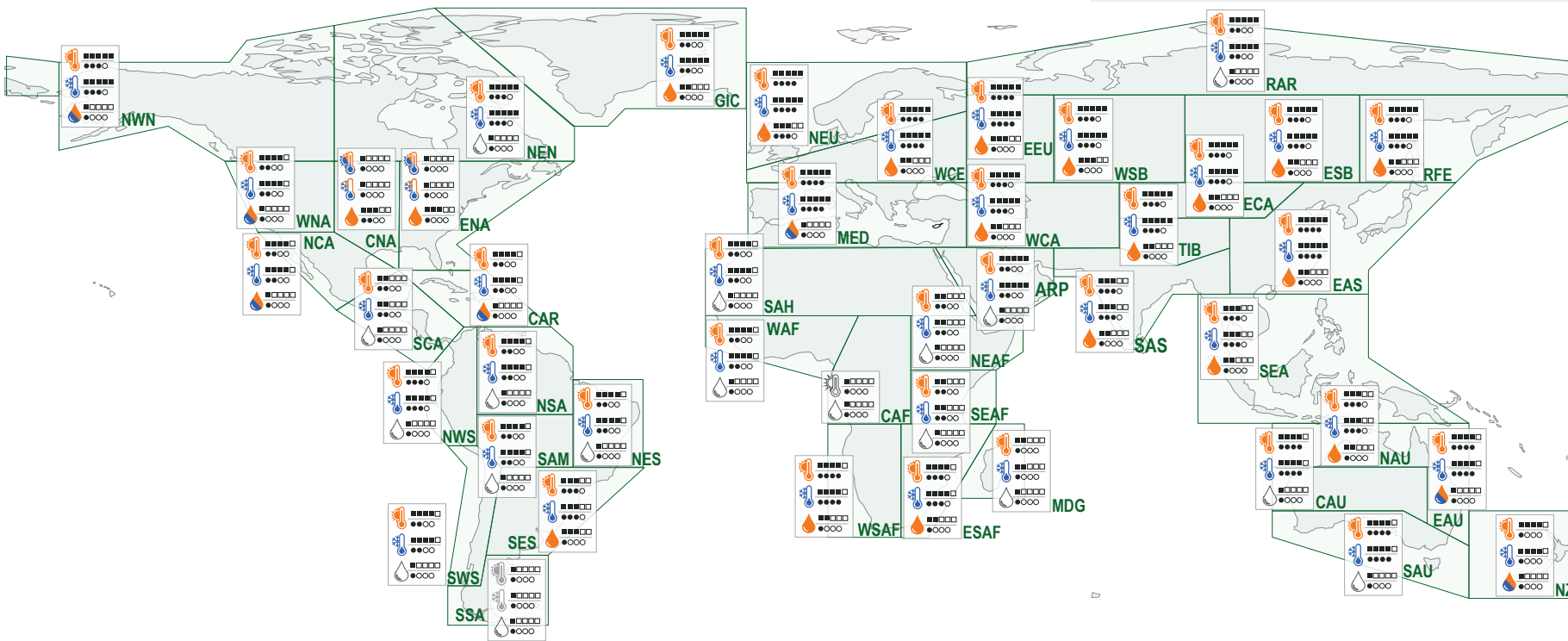
Figure 11.4 | Overview of observed changes for cold, hot, and wet extremes and their potential human contribution. Shown are the direction of change and the confidence in: 1) the observed changes in cold and hot as well as wet extremes across the world; and 2) whether human-induced climate change contributed to causing these changes (attribution). In each region changes in extremes are indicated by colour (orange – increase in the type of extreme; blue – decrease; both colours – changes of opposing direction within the region, with the signal depending on the exact event definition; grey – there are no changes observed; and no fill – the data/evidence is too sparse to make an assessment). The squares and dots next to the symbol indicate the level of confidence for observing the trend and the human contribution, respectively. The more black dots/squares, the higher the level of confidence. The information on this figure is based on regional assessment of the literature on observed trends, detection and attribution and event attribution in Section 11.9.
