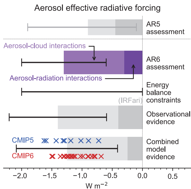
Figure 7.5 | Net aerosol effective radiative forcing (ERF) from different lines of evidence. The headline AR6 assessment of -1.3 [ -2.0 to -0.6 ] \text{W m}^{-2} is highlighted in purple for 1750–2014 and compared to the AR5 assessment of -0.9 [ -1.9 to -0.1 ] \text{W m}^{-2} for 1750–2011. The evidence comprising the AR6 assessment is shown below this: energy balance constraints [ -2 to 0 \text{ W m}^{-2} with no best estimate]; observational evidence from satellite retrievals of -1.4 [ -2.2 to -0.6 ] \text{W m}^{-2} ; and climate model-based evidence of -1.25 [ -2.1 to -0.4 ] \text{W m}^{-2} . Estimates from individual CMIP5 (Zelinka et al., 2014) and CMIP6 (Smith et al., 2020b and Table 7.6) models are depicted by blue and red crosses respectively. For each line of evidence the assessed best-estimate contributions from ERF ari and ERF aci are shown with darker and paler shading respectively. The observational assessment for ERF ari is taken from the IRF ari . Uncertainty ranges are represented by black bars for the total aerosol ERF and depict very likely ranges. Further details on data sources and processing are available in the chapter data table (Table 7.SM.14).
