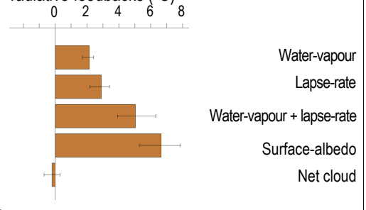
Arctic warming contributions from individual radiative feedbacks (°C)
