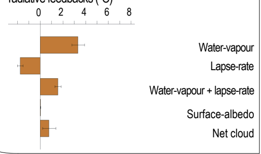
Tropics warming contributions from individual radiative feedbacks (°C)
