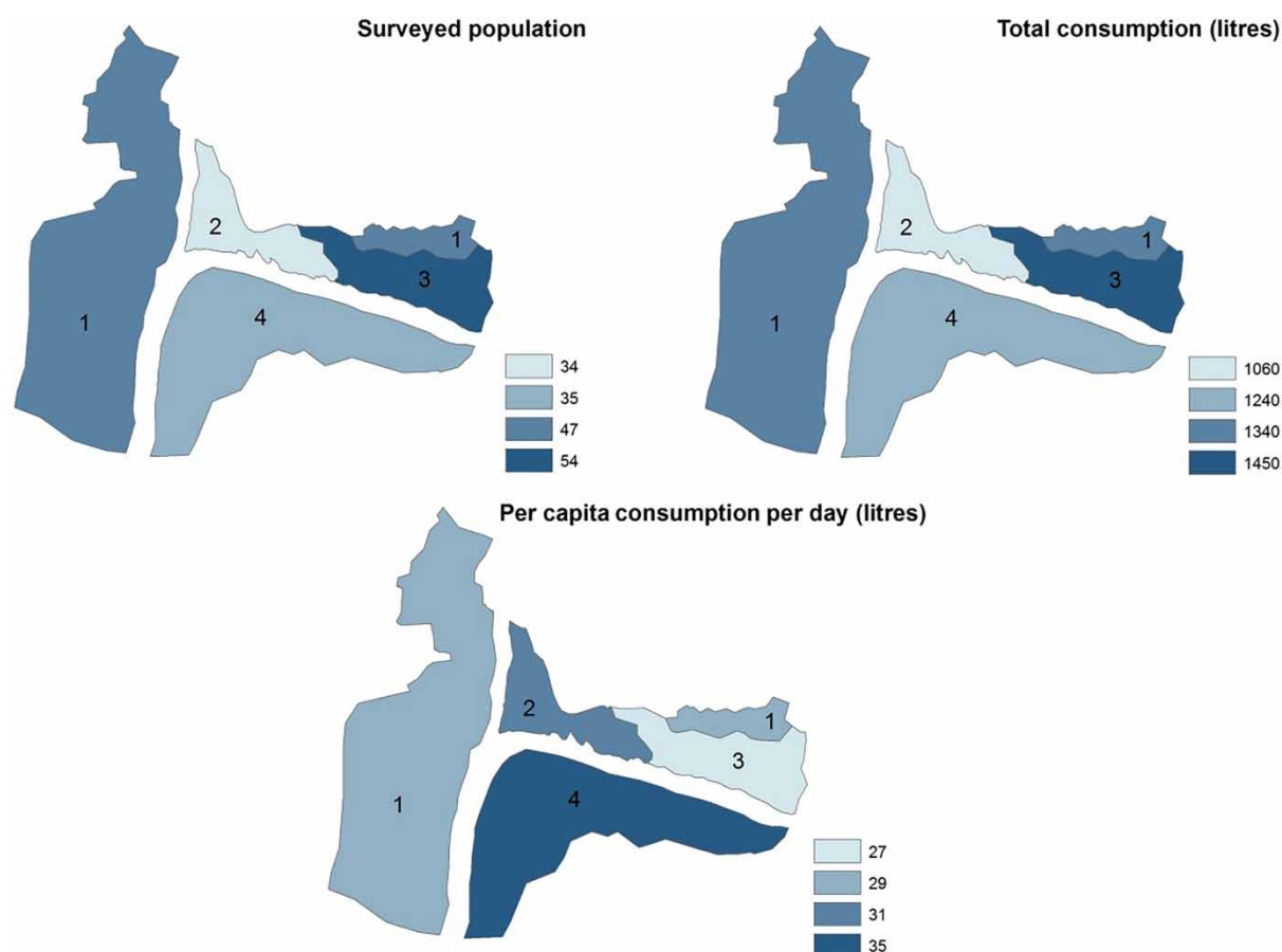
Fig. 9. Ward-wise water consumption in Devprayag.
