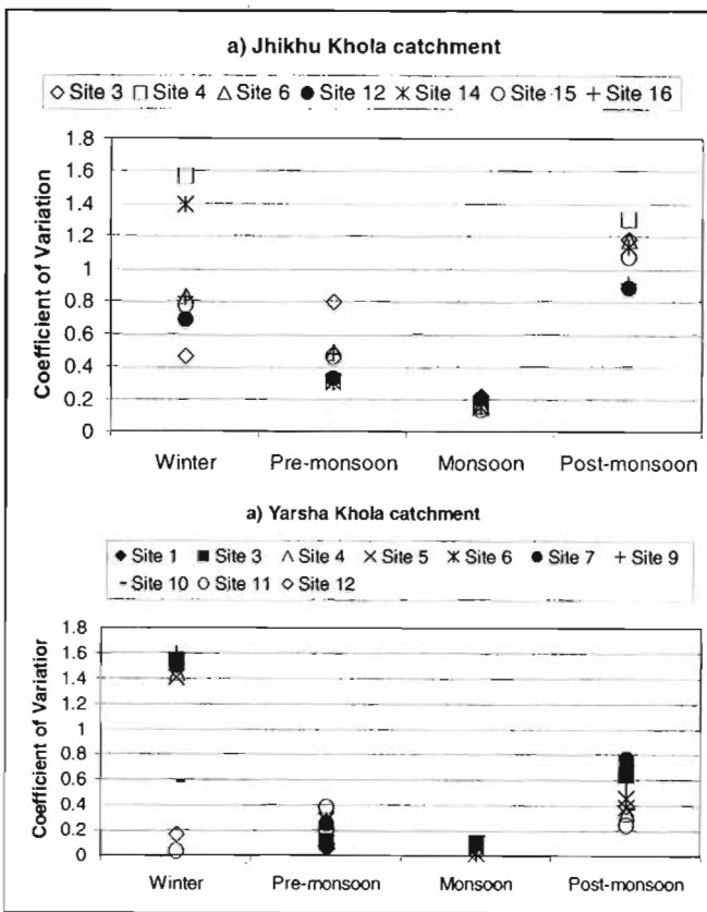
Figure 9.1: Seasonal rainfall variability in the Jhikhu Khola (1993-2000) and Yarsha Khola (1998-2000) catchments
