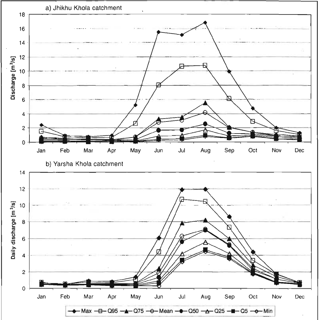
Figure 9.3: Runoff regime at main stations in the Jhikhu Khola and Yarsha Khola catchments
