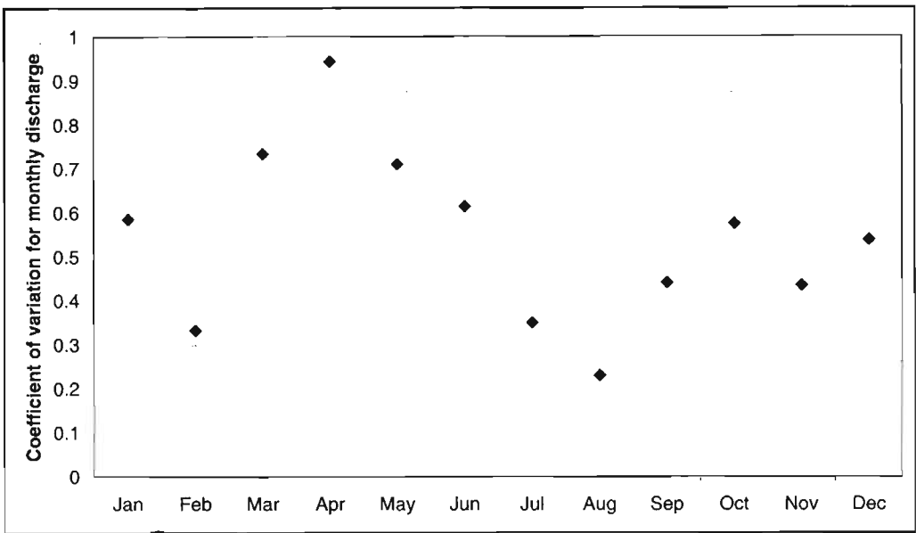
Figure 9.4: Temporal variability of monthly flows for the Jhikhu Khola catchment
