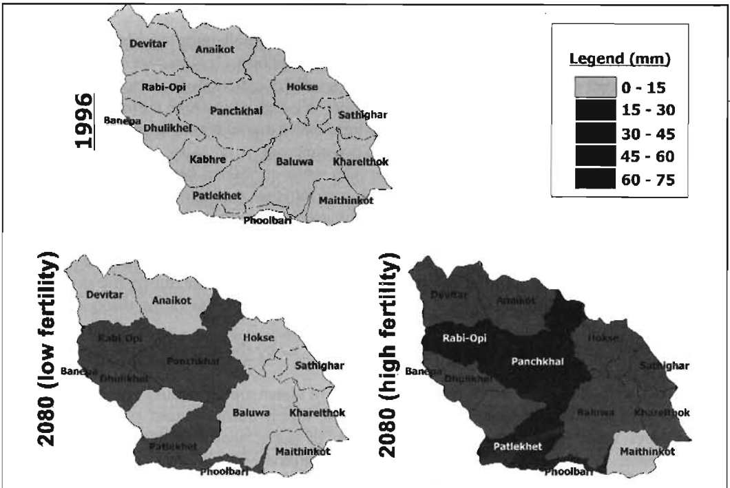
Figure 9.9: Projected water demand 1996-2080 in Jhikhu Khola VDCs
