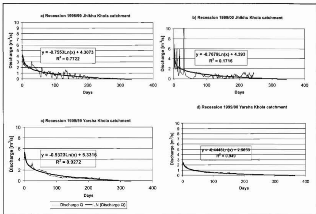
Figure 9.6: Flow recession curves in the Jhikhu Khola catchment: a) 1998/1999 dry season, b) 1999/2000 dry season; and for the Yarsha Khola catchment: c) 1998/1999 dry season, and d) 1999/2000 dry season.
