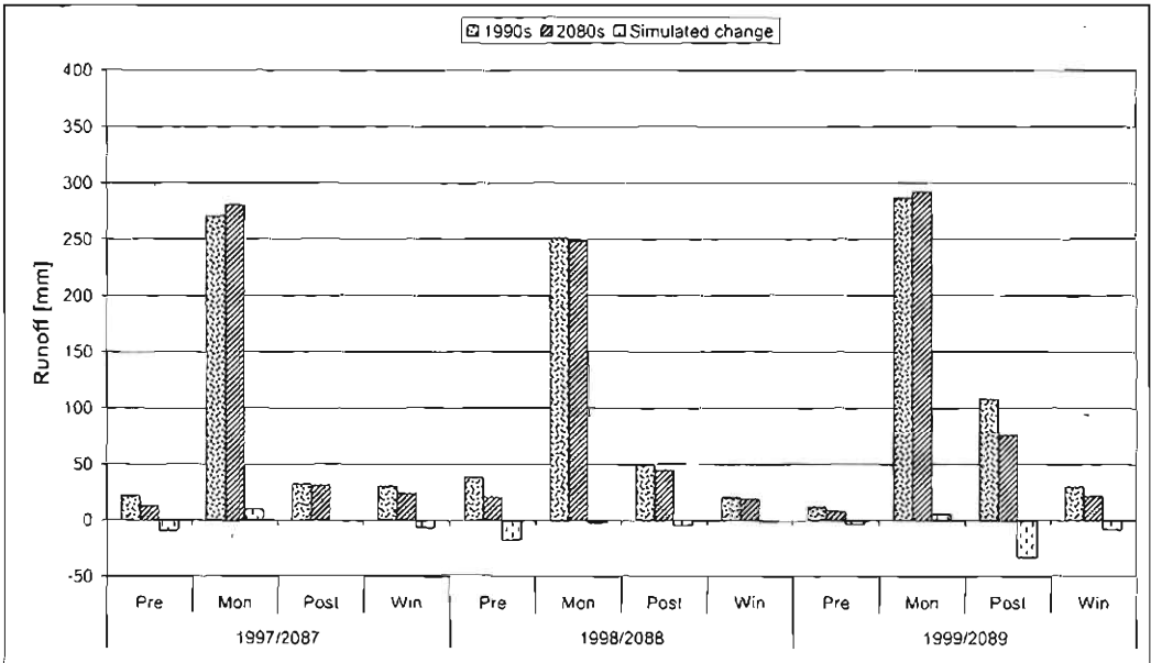
Figure 9.8: Seasonal changes of runoff from the Jhikhu Khola catchment with global climate change determined by applying PREVAH model (Merz 2004)
