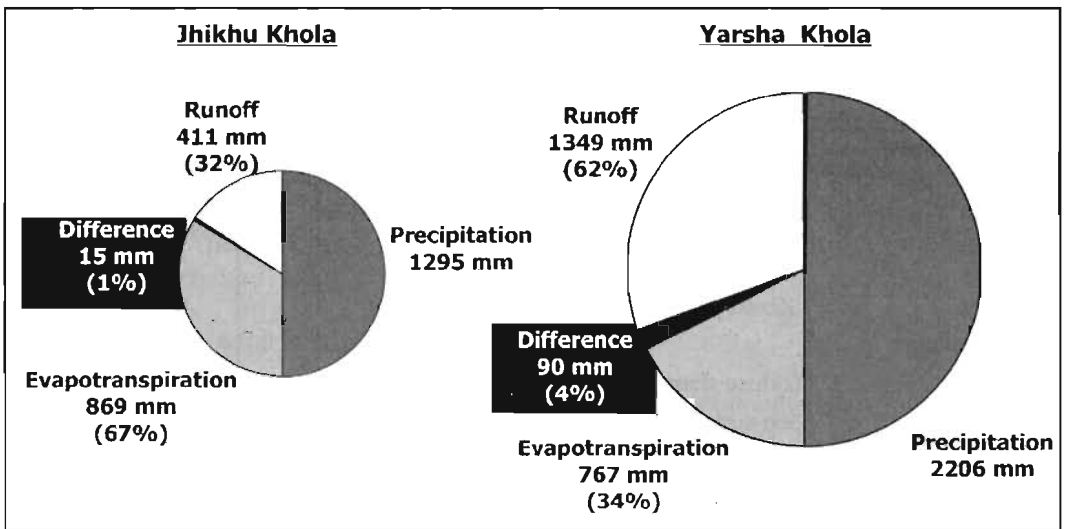
Figure 9.7: Hydrological water balance of the Jhikhu and Yarsha Khola catchments
