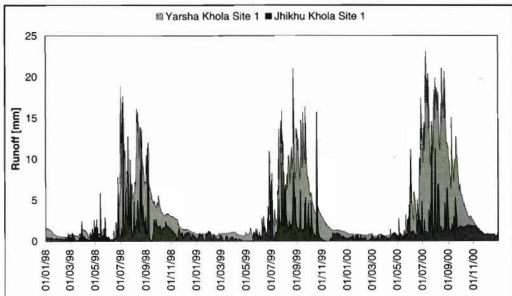
Figure 9.5: Comparison of daily runoff at the outlets of Yarsha Khola and Jhikhu Khola
