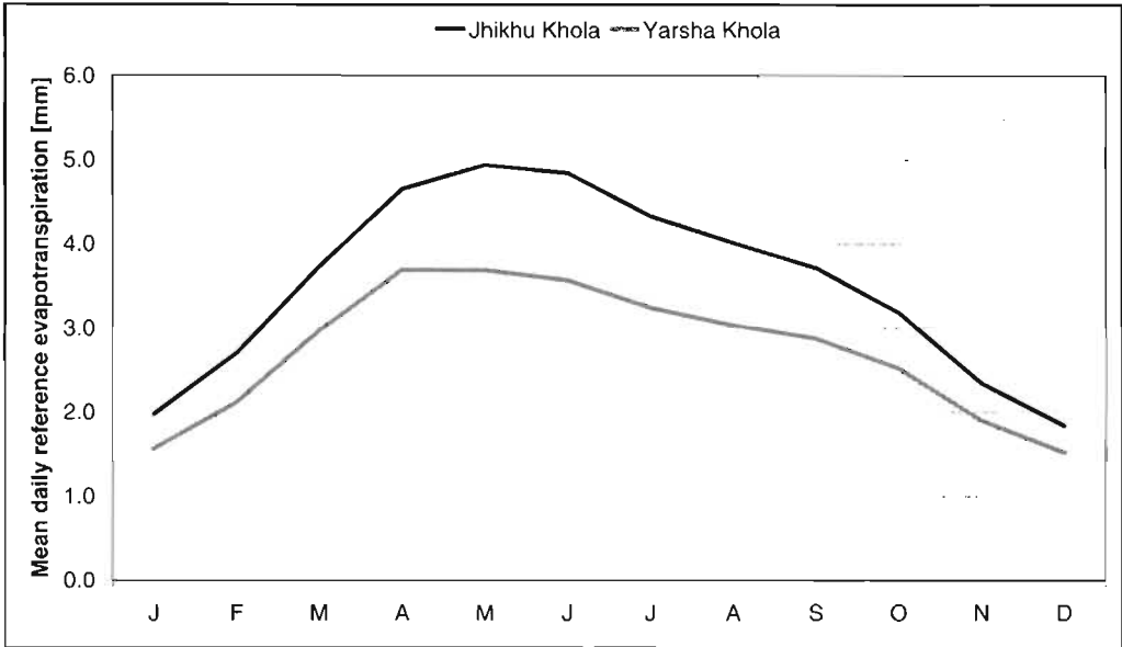
Figure 9.2: Mean daily reference evapotranspiration at main stations of Jhikhu Khola and Yarsha Khola catchments
